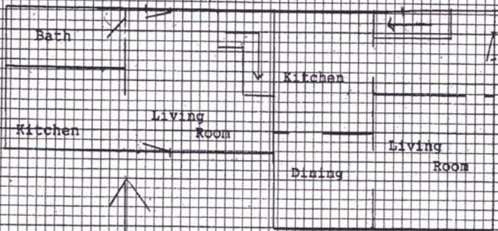
First Floor Layout
